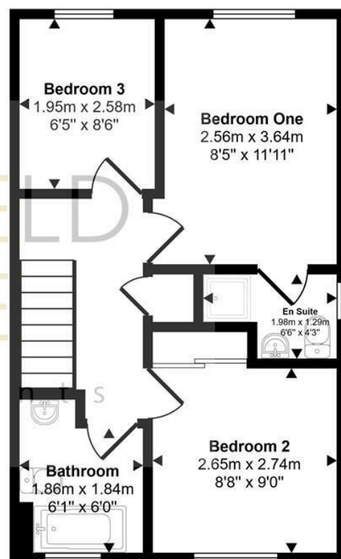
First Floor Approx 37 sq m / 400 sq ft
